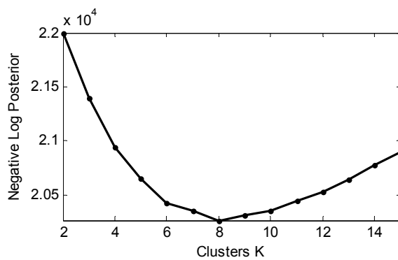
Fig. 7. Results of the cluster number selection process in the objective classification. The horizontal axis is the number of clusters, and the vertical axis is the negative log posterior.
