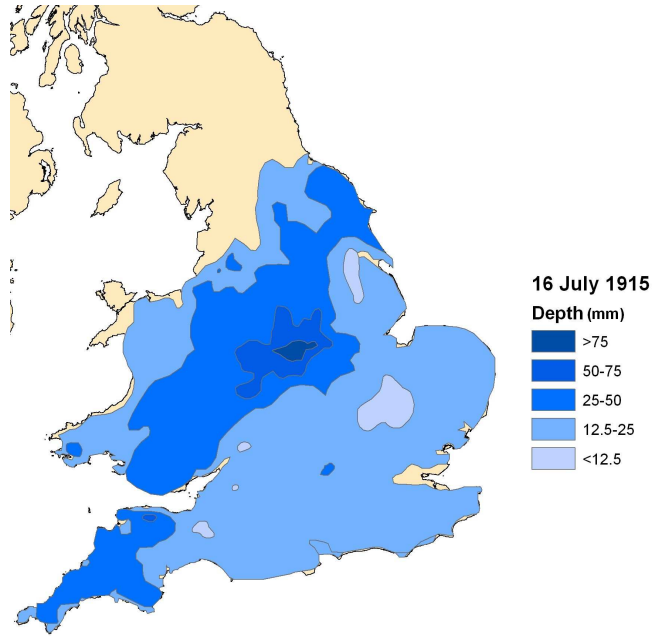
Fig. 1. Typical depression extreme rainfall event identified from the British Rainfall archive.
